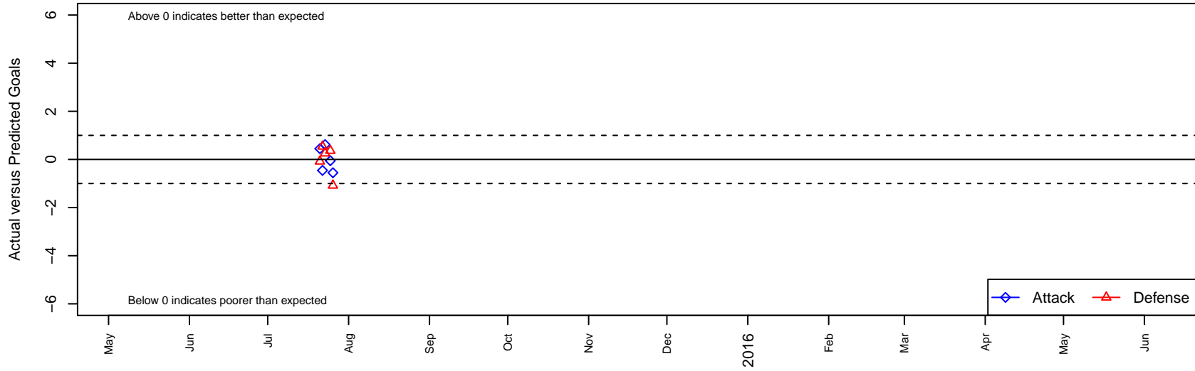
GOL GSA 01 Premier B00 Dots are actual minus expected GF (blue circles) and GA (red triangles). Blue line is smoothed change in attack strength. Red is smoothed change in defense strength.
